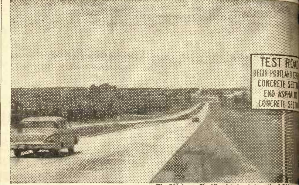
The Oklahoma Test Road is located north of Oklahoma City.
